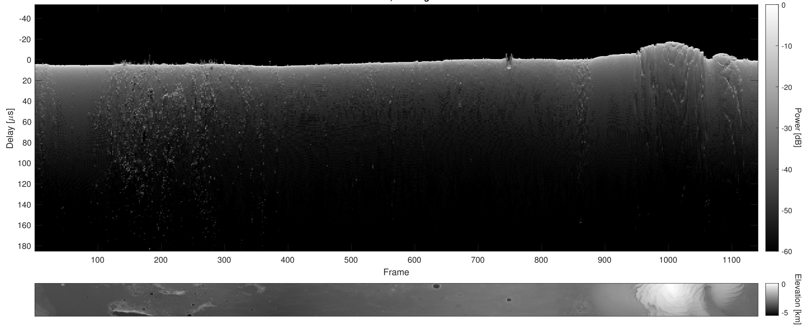
Orbit 3795, Cluttergram
