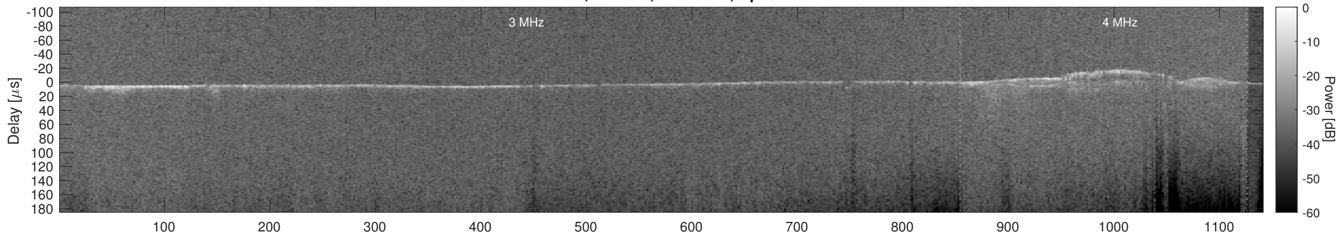
Orbit 3795, Cluttergram
