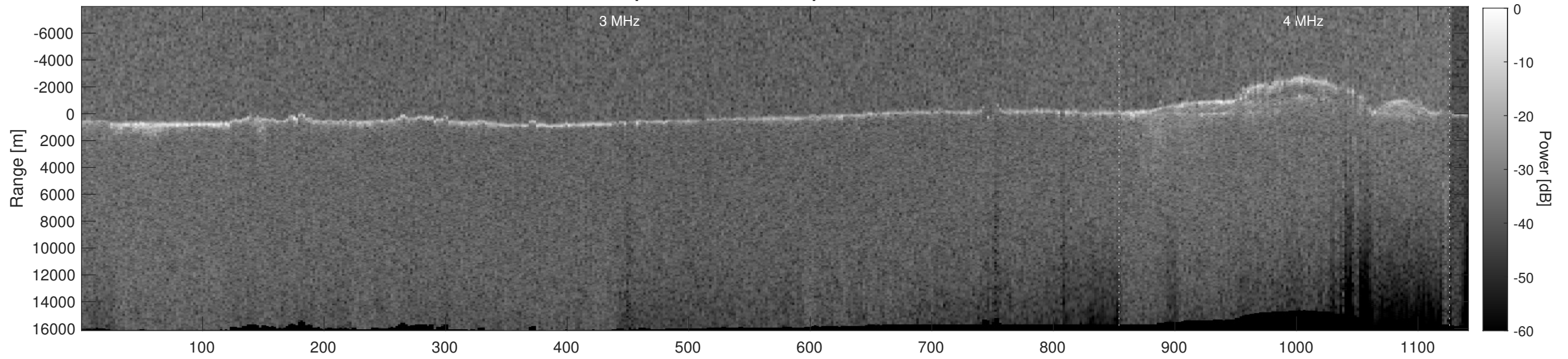
Orbit 3795, Depth-Corrected Cluttergram
