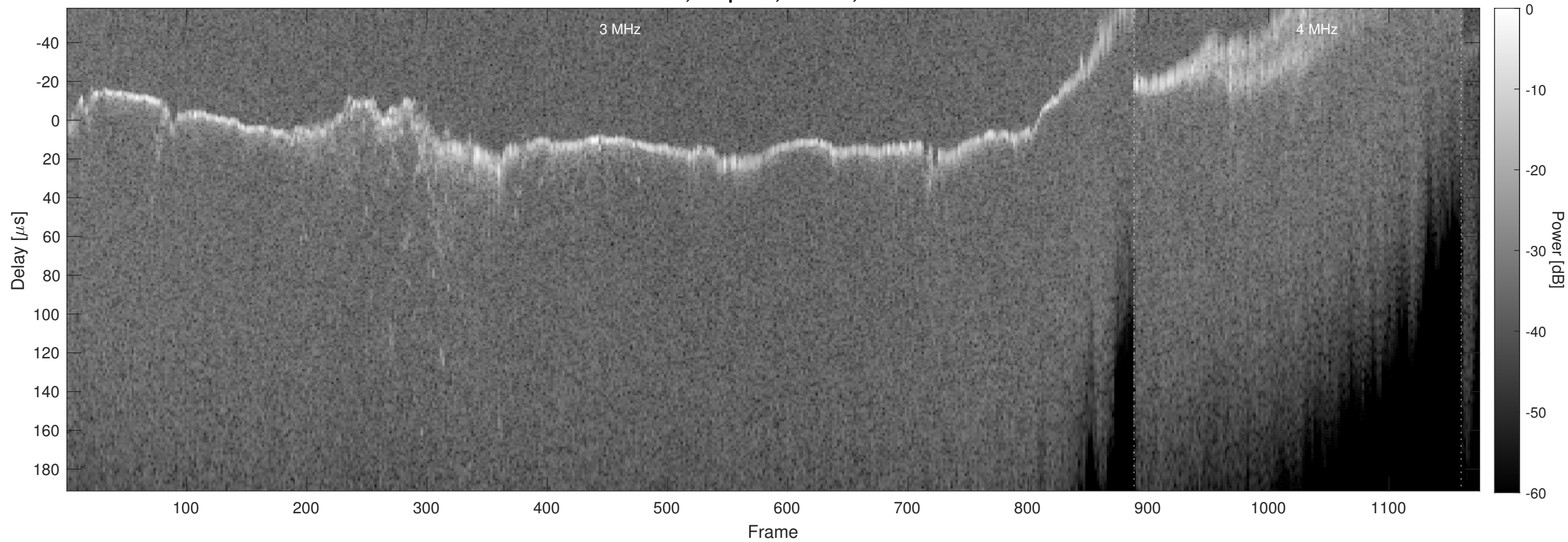
Orbit 3796, Chapman, Window, Channel 2
