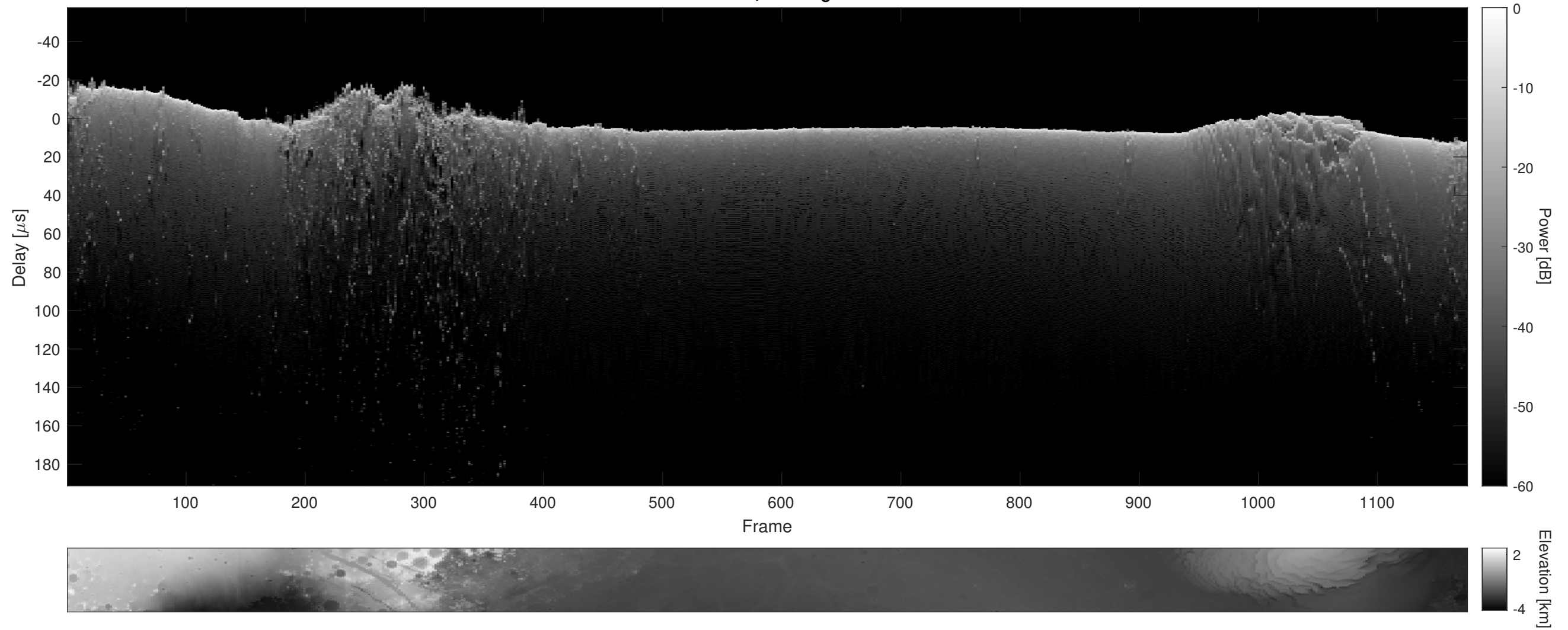
Orbit 3796, Cluttergram
