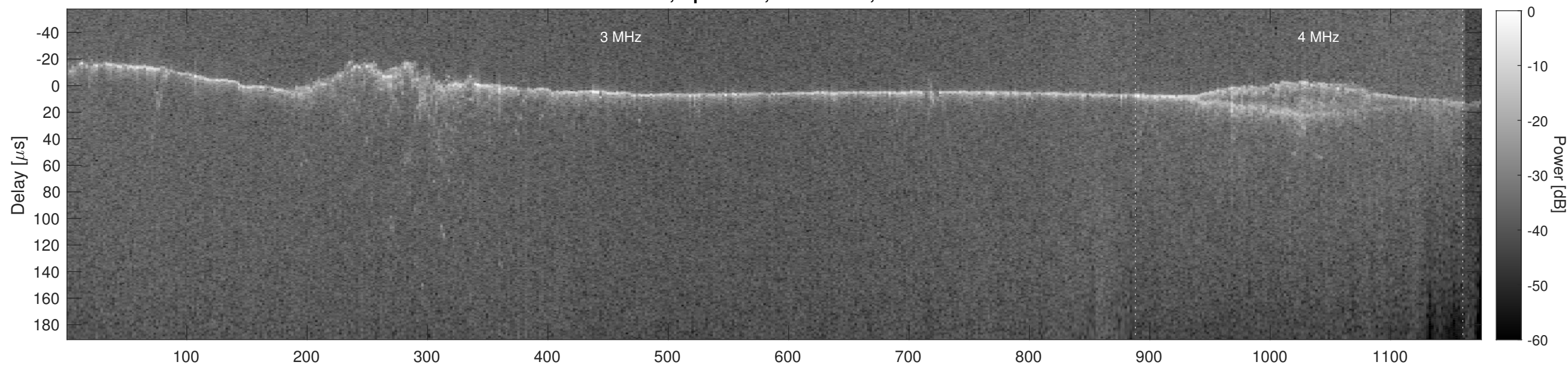
Orbit 3796, Cluttergram
