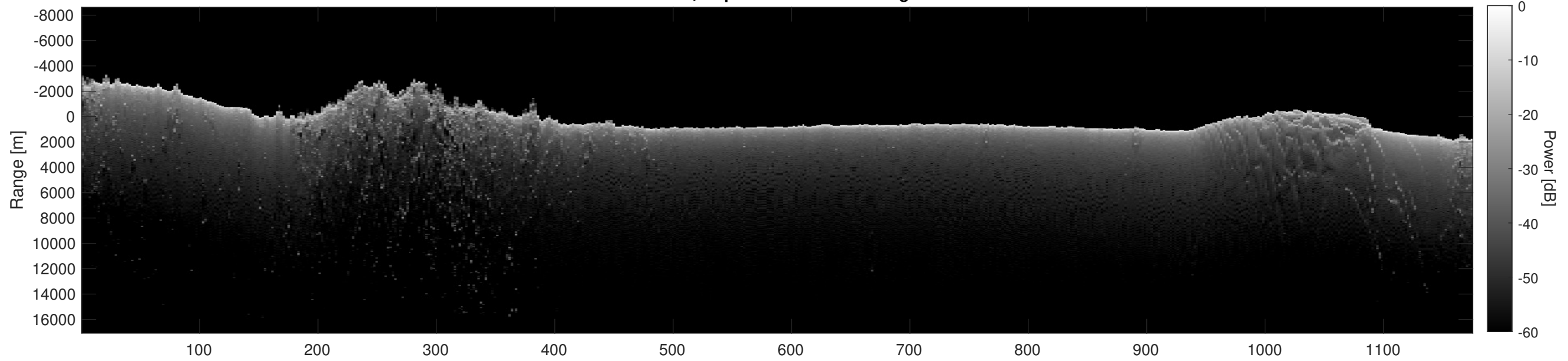
Orbit 3796, Depth-Corrected Cluttergram
