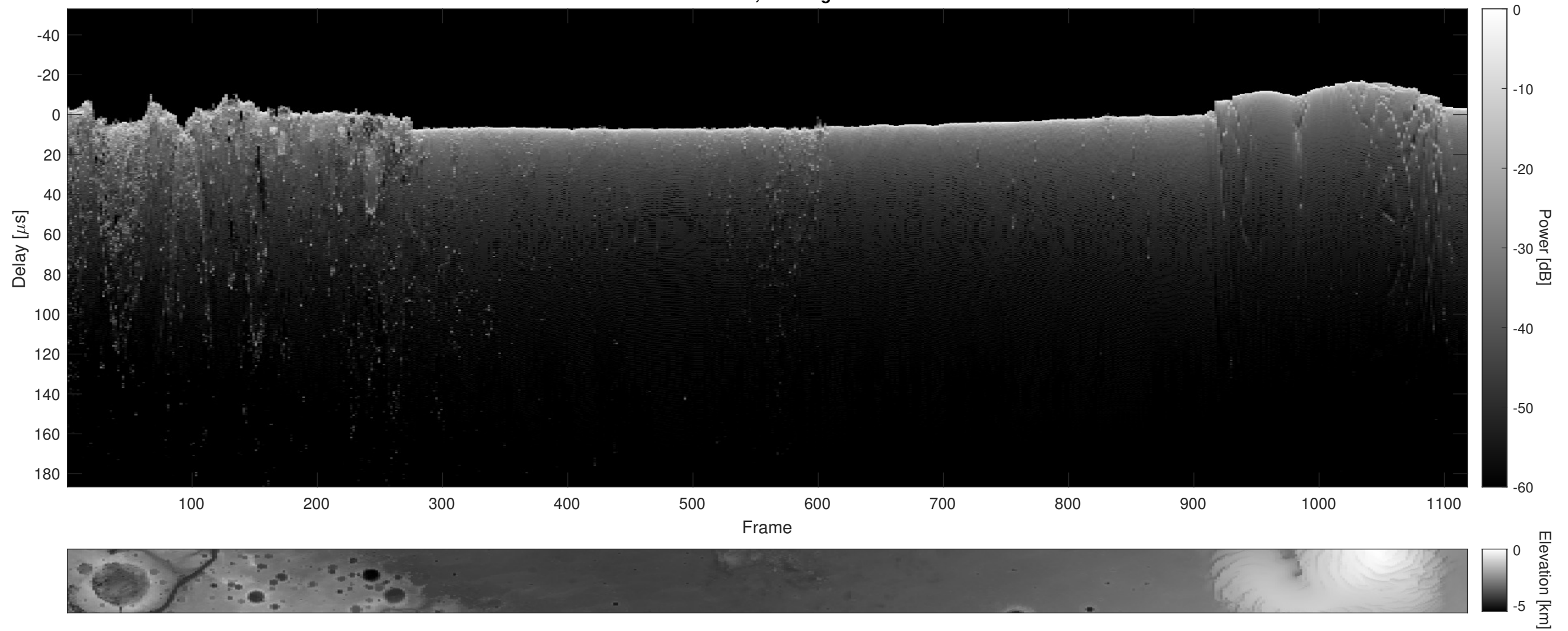
Orbit 3797, Cluttergram
