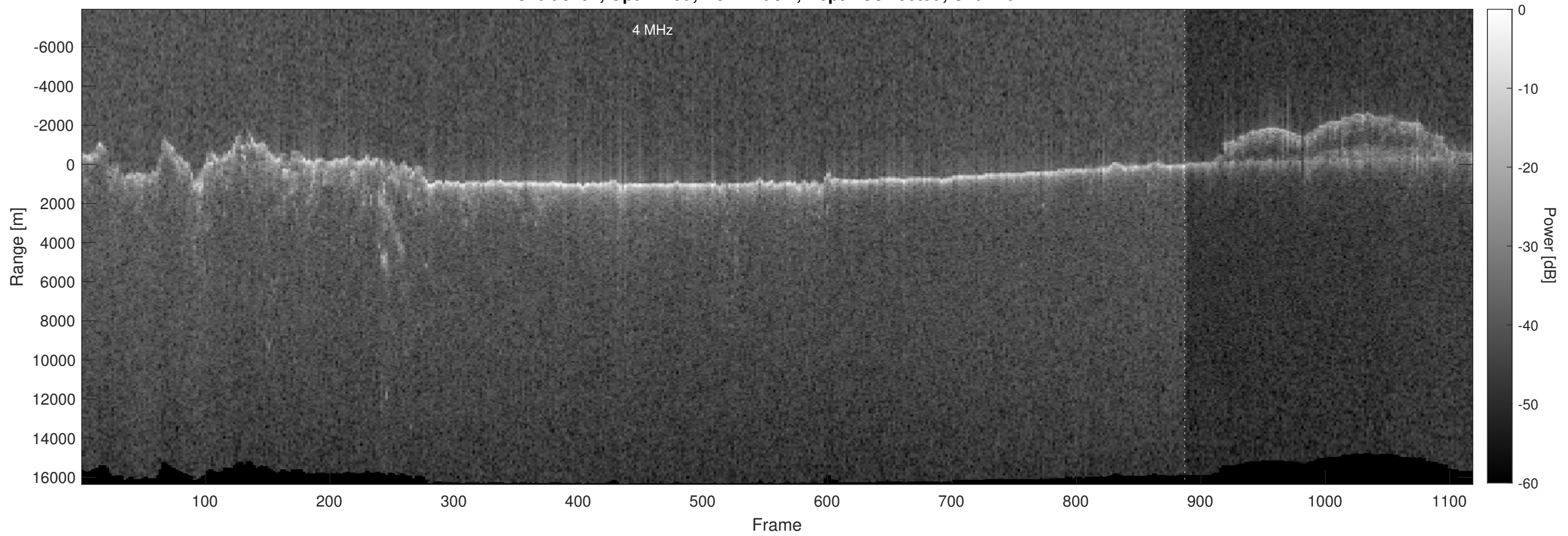
Orbit 3797, Optimized, No Window, Depth-Corrected, Channel 2
