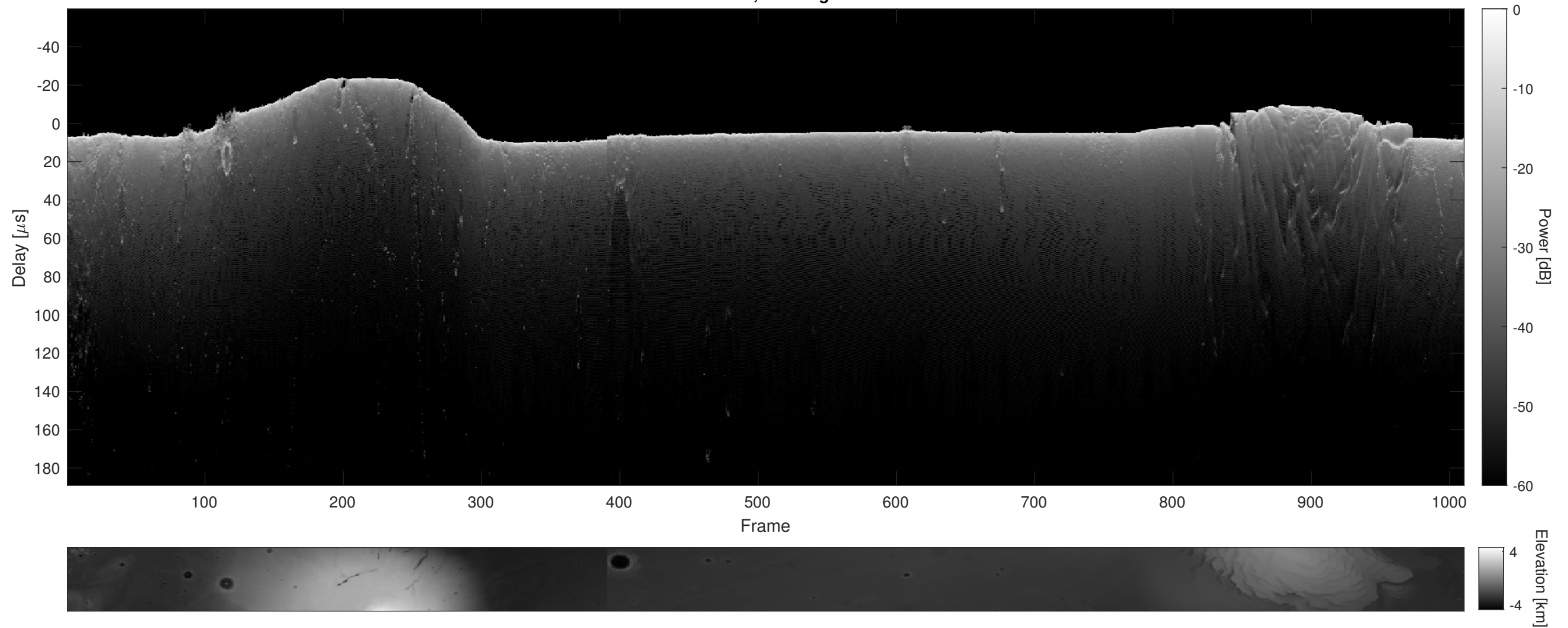
Orbit 3799, Cluttergram
