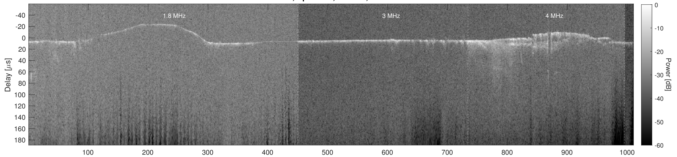
Orbit 3799, Cluttergram
