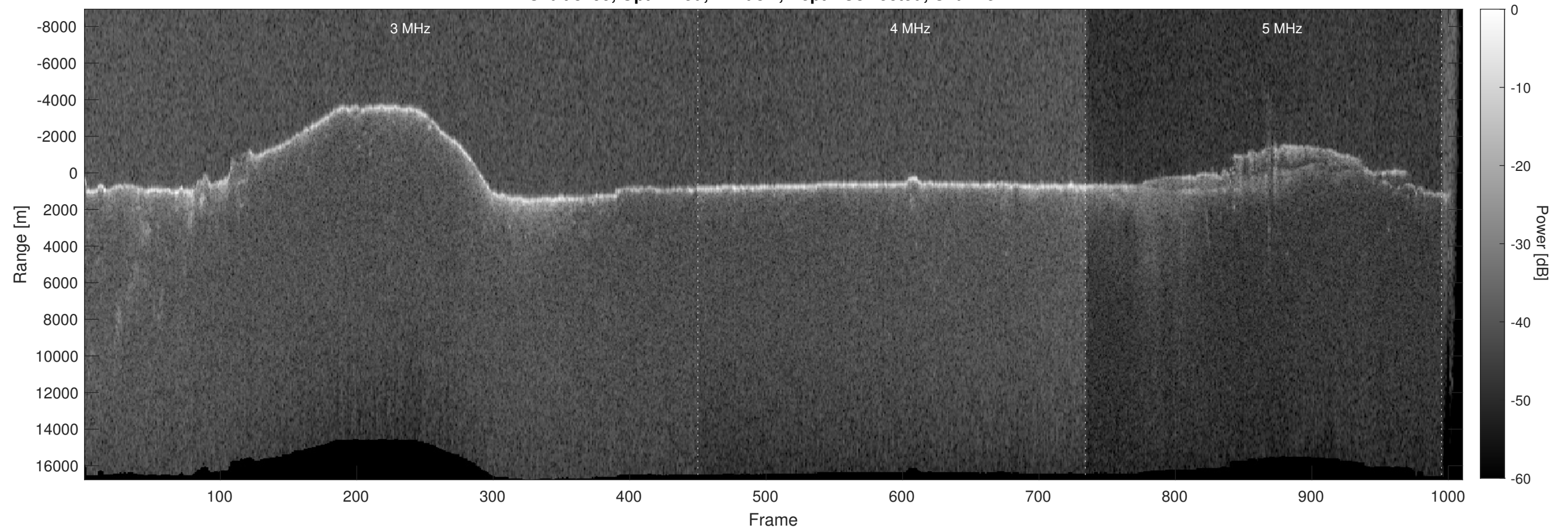
Orbit 3799, Optimized, Window, Depth-Corrected, Channel 2
