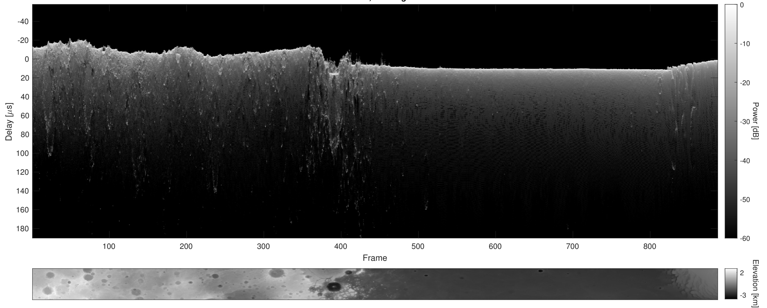
Orbit 3800, Cluttergram
