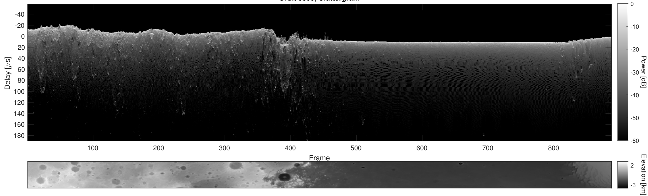
Orbit 3800, Cluttergram
