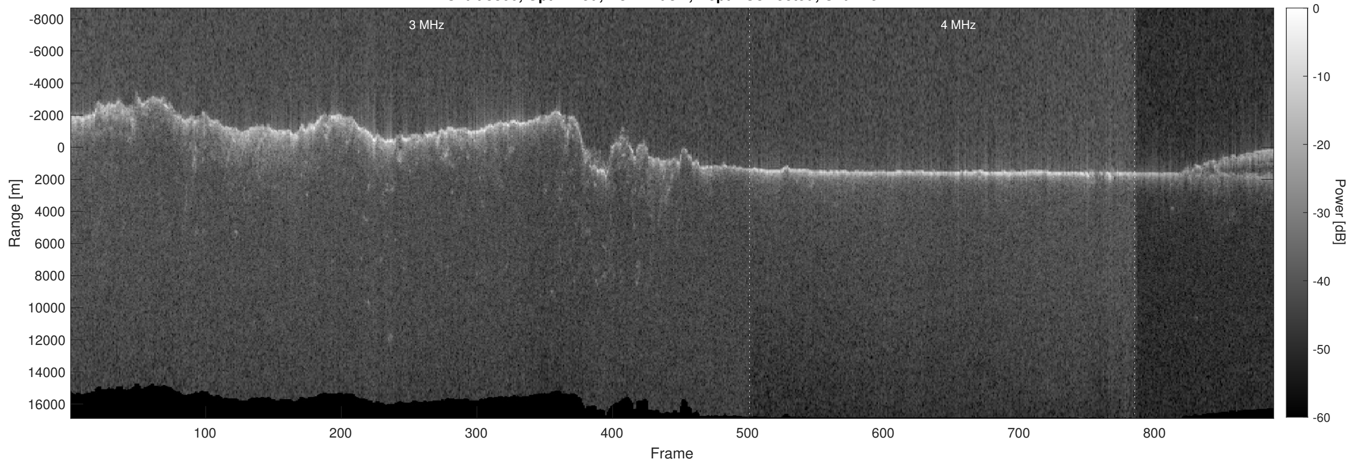
Orbit 3800, Optimized, No Window, Depth-Corrected, Channel 2
