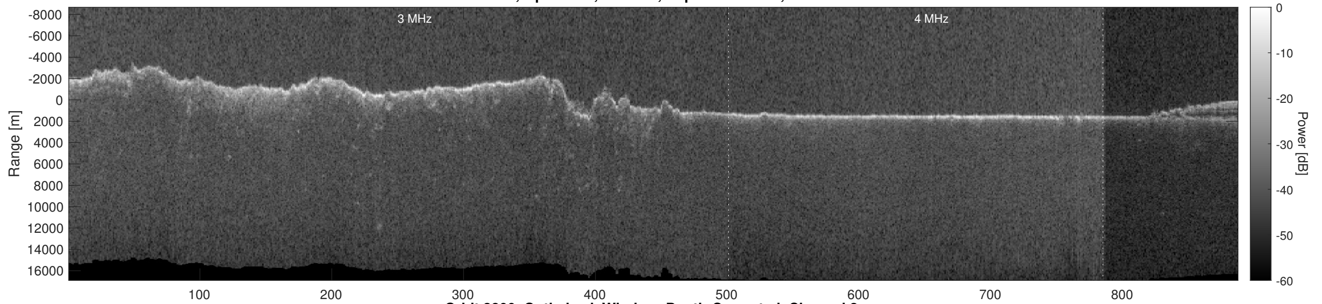
Orbit 3800, Optimized, Window, Depth-Corrected, Channel 2
