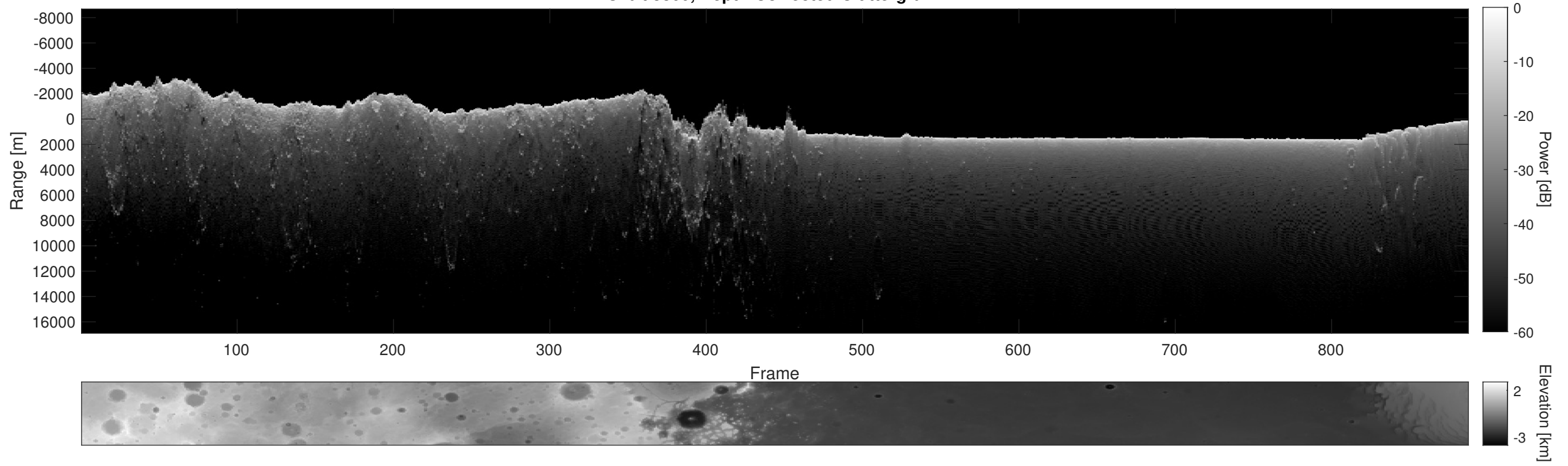
Orbit 3800, Depth-Corrected Cluttergram
