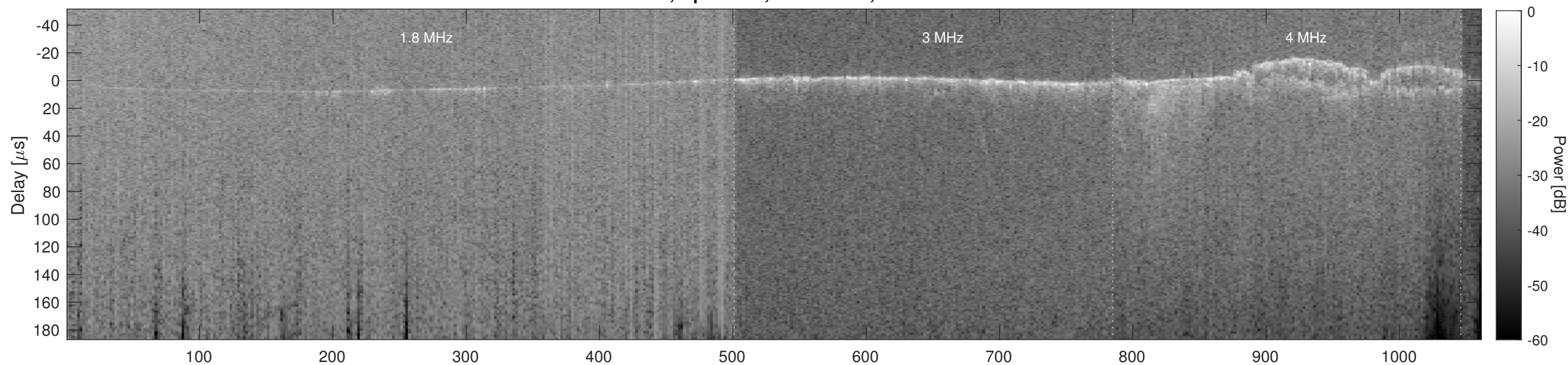
Orbit 3802, Cluttergram
