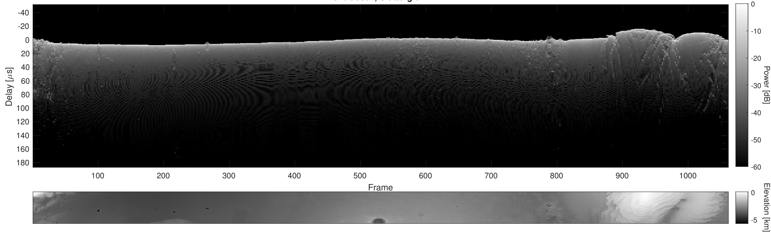
Orbit 3802, Cluttergram
