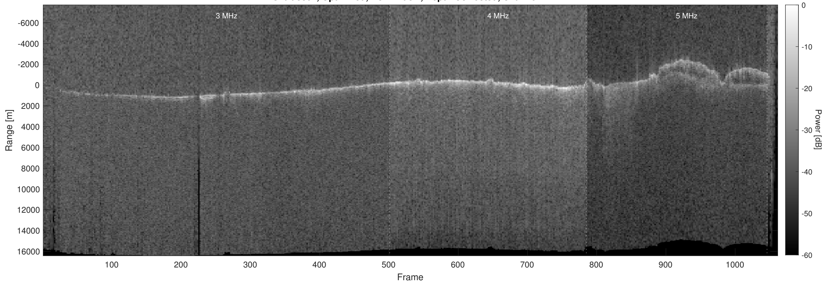
Orbit 3802, Optimized, No Window, Depth-Corrected, Channel 2
