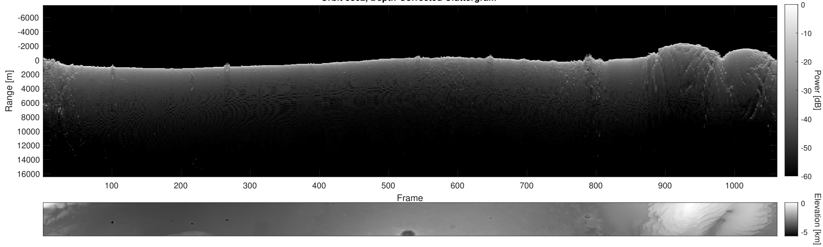
Orbit 3802, Depth-Corrected Cluttergram
