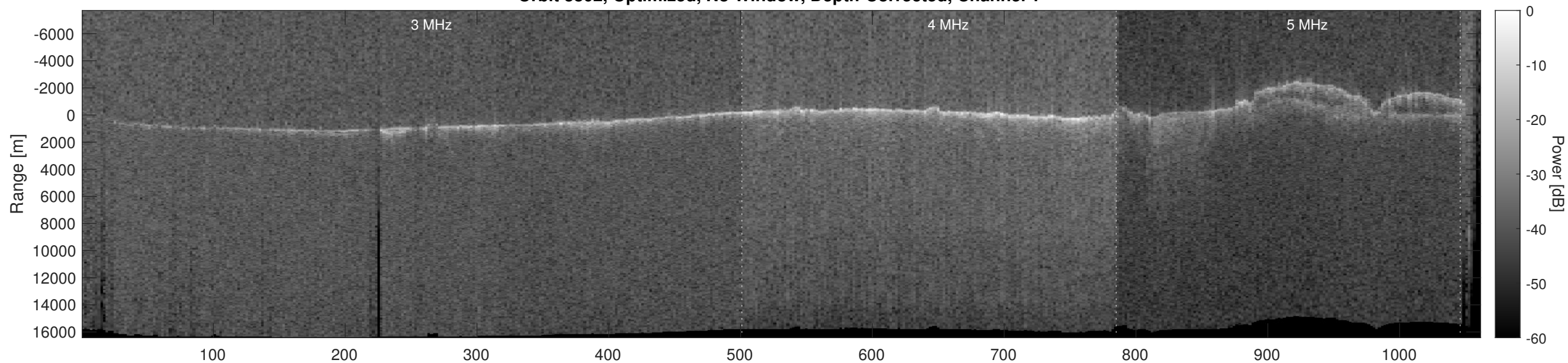
Orbit 3802, Optimized, No Window, Depth-Corrected, Channel 2
