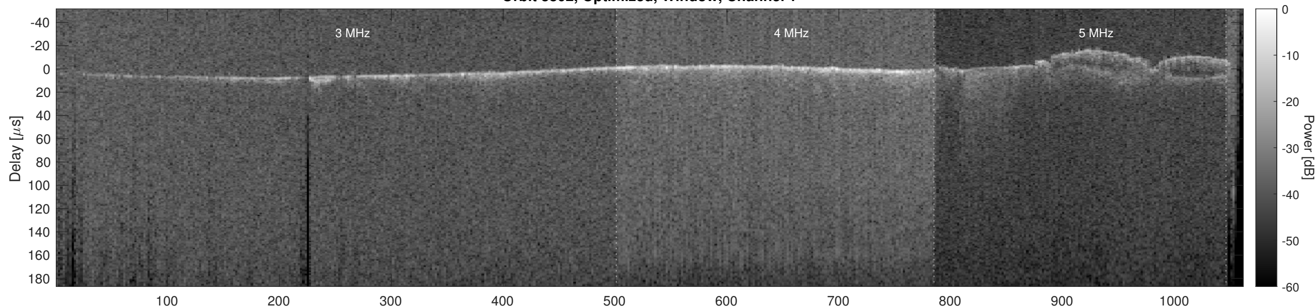
Orbit 3802, Optimized, Window, Channel 2
