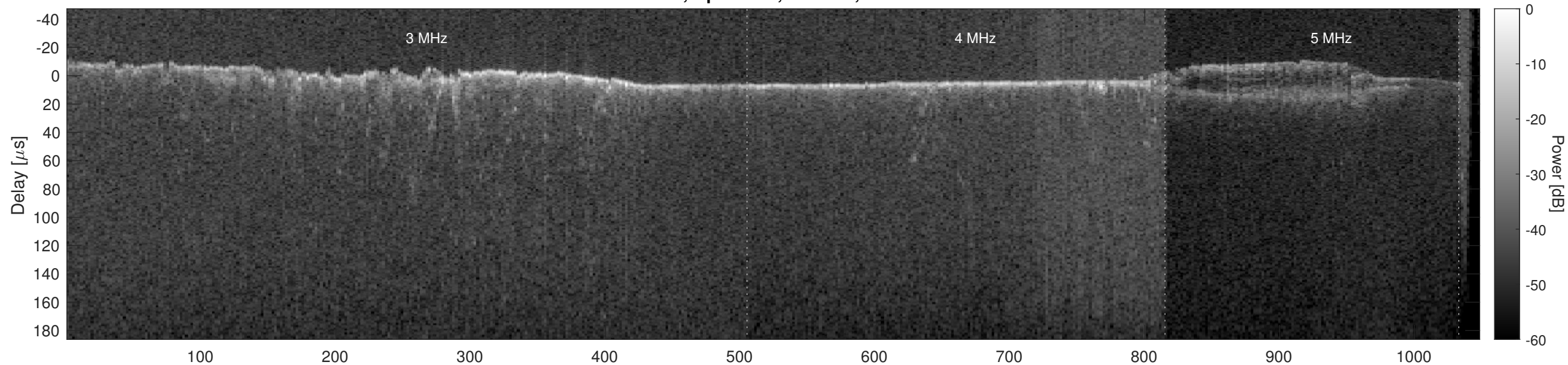
Orbit 3804, Optimized, Window, Channel 2
