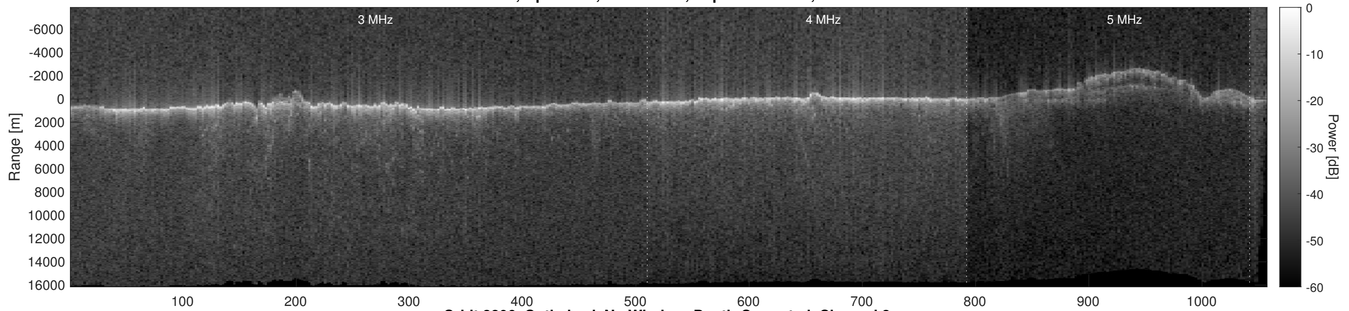
Orbit 3806, Optimized, No Window, Depth-Corrected, Channel 2
