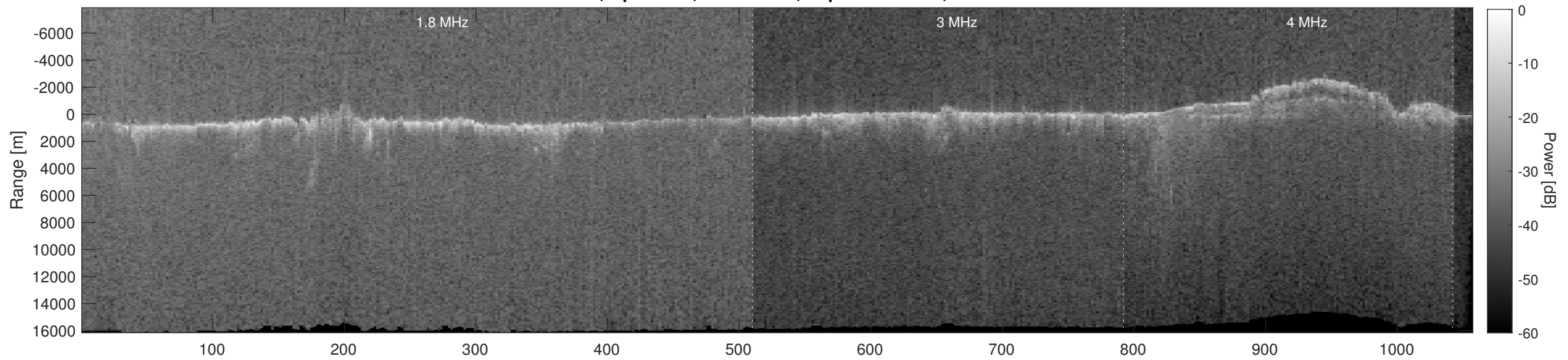
Orbit 3806, Depth-Corrected Cluttergram
