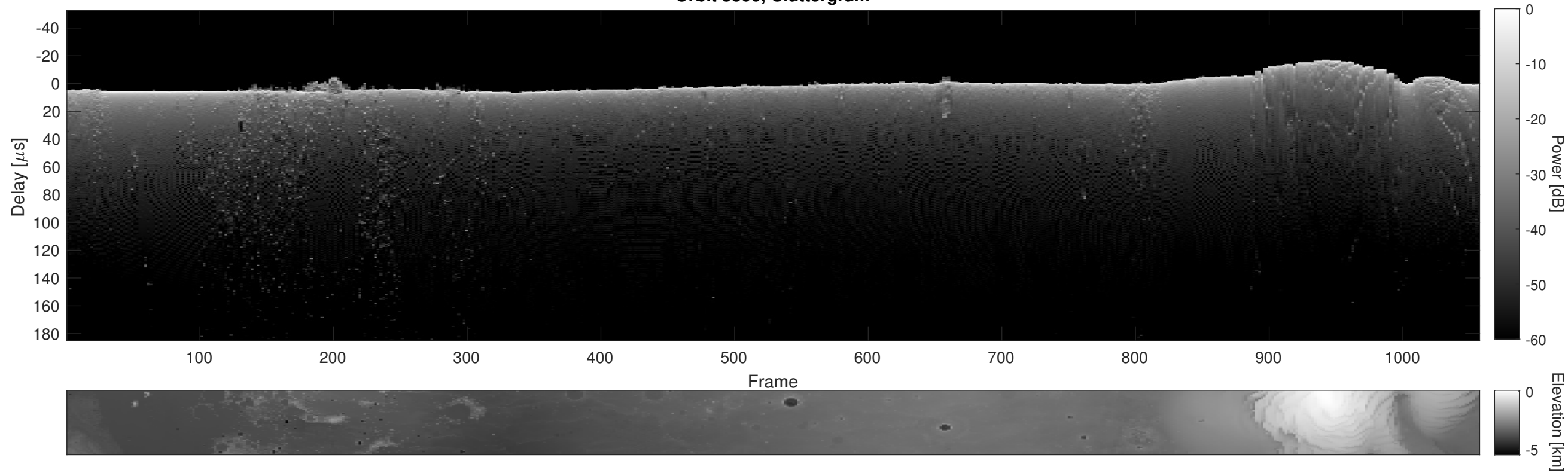
Orbit 3806, Cluttergram
