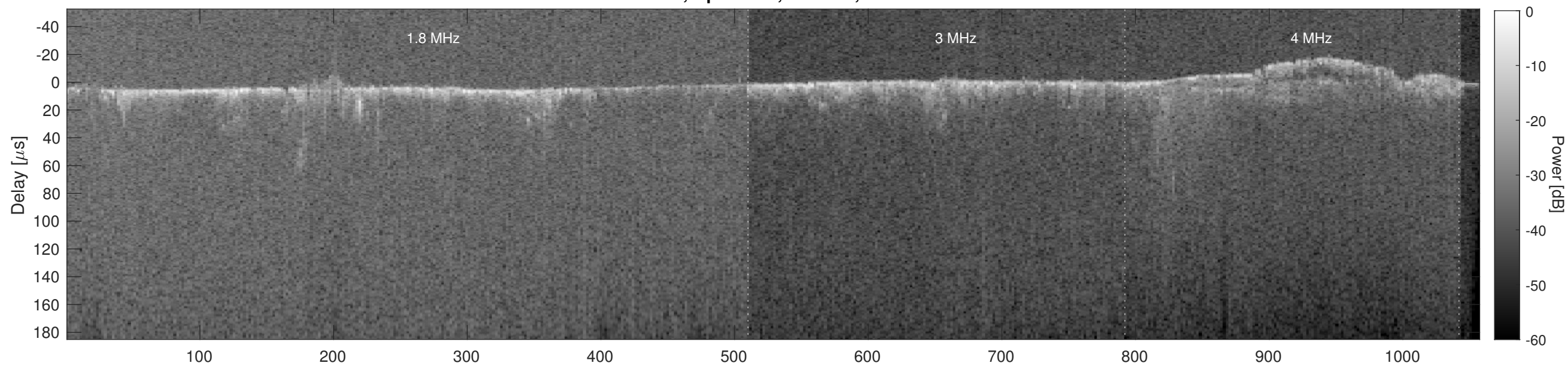
Orbit 3806, Cluttergram
