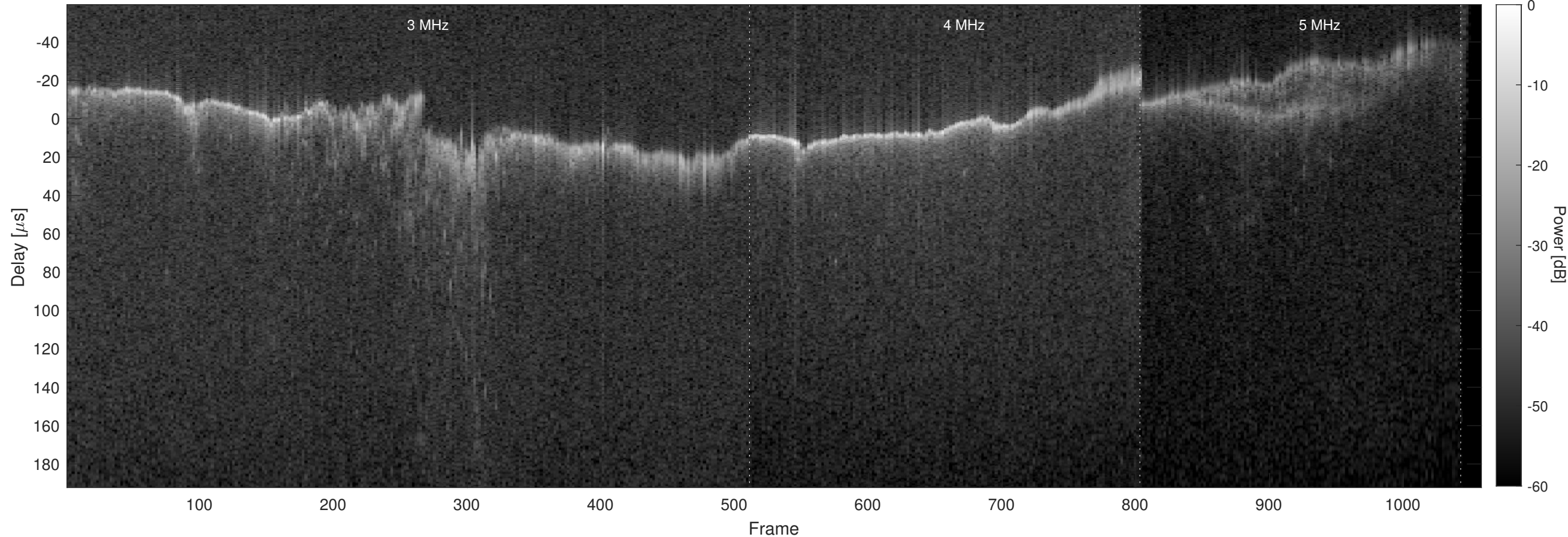
Orbit 3807, Chapman, No Window, Channel 2
