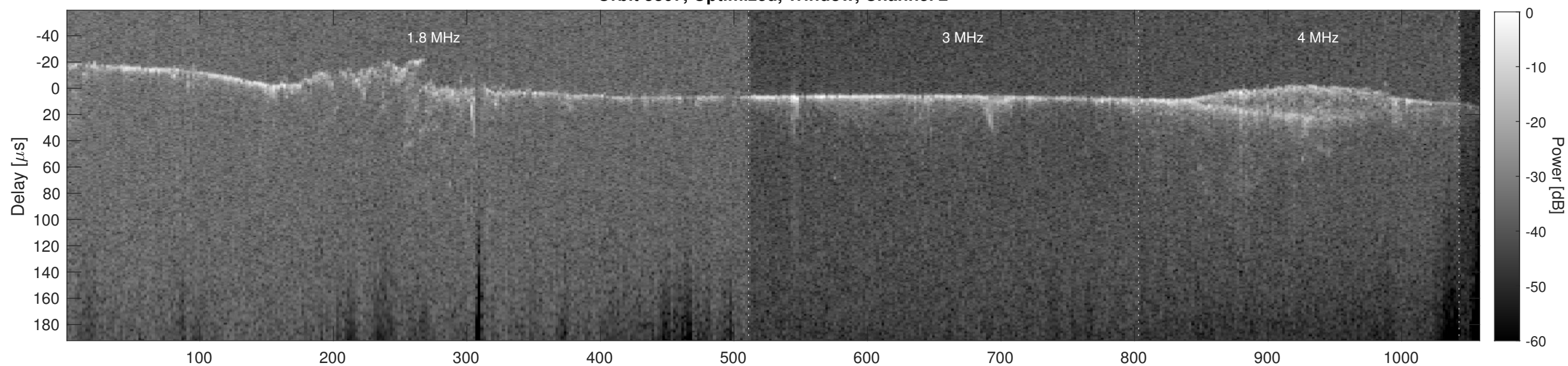
Orbit 3807, Cluttergram
