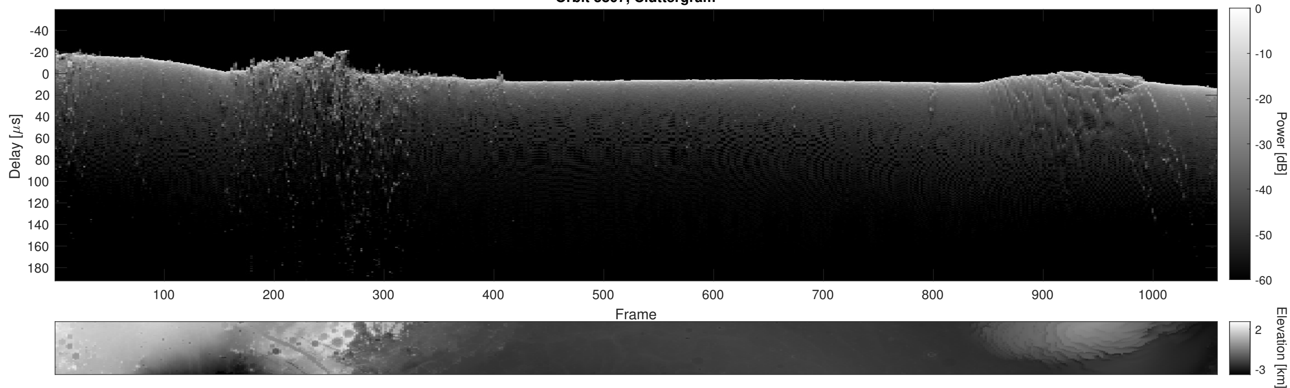
Orbit 3807, Cluttergram
