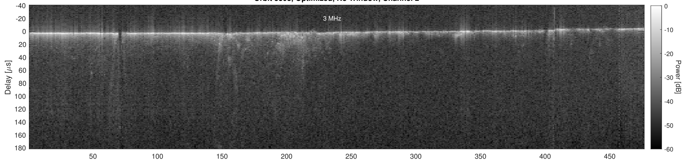
Orbit 3808, Cluttergram
