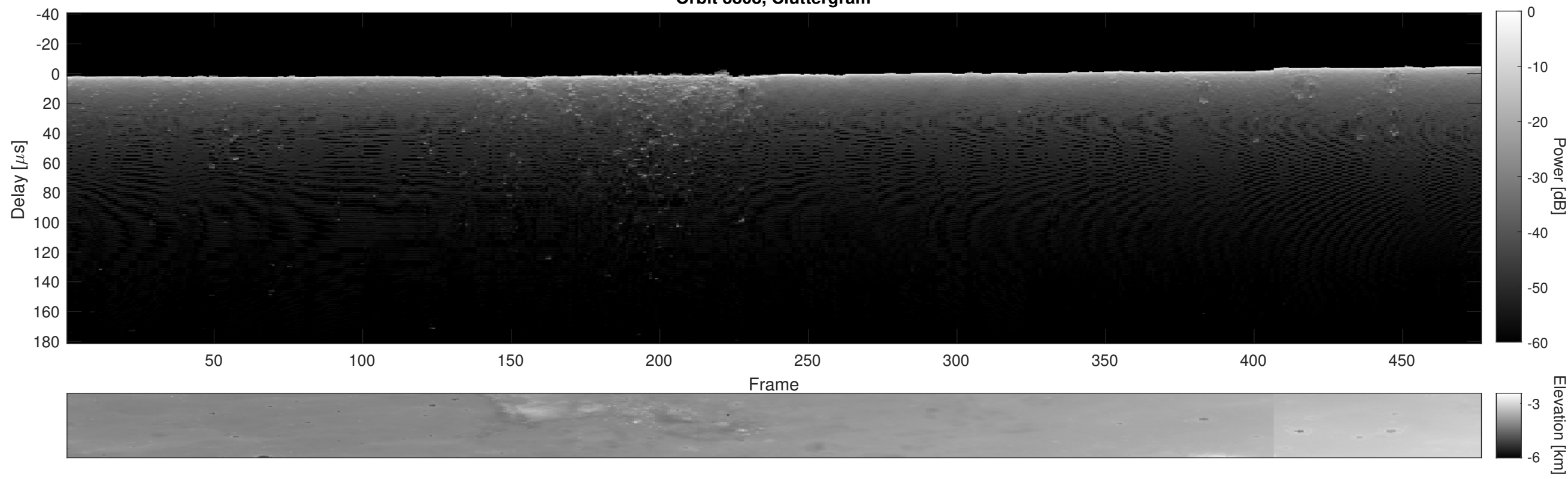
Orbit 3808, Cluttergram
