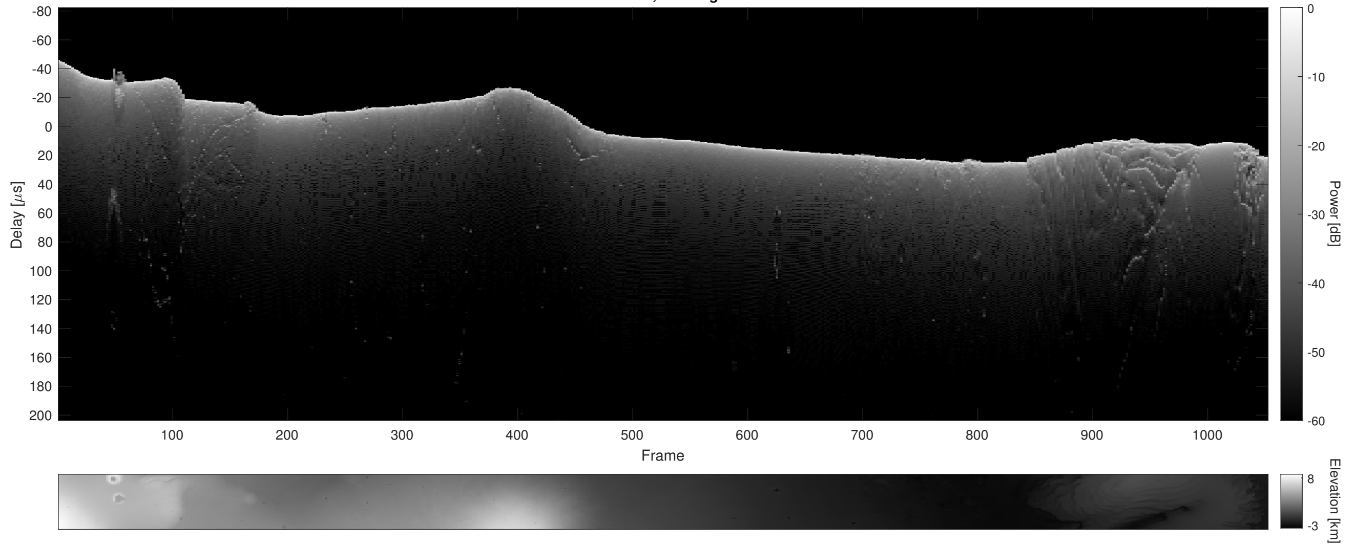
Orbit 3809, Cluttergram
