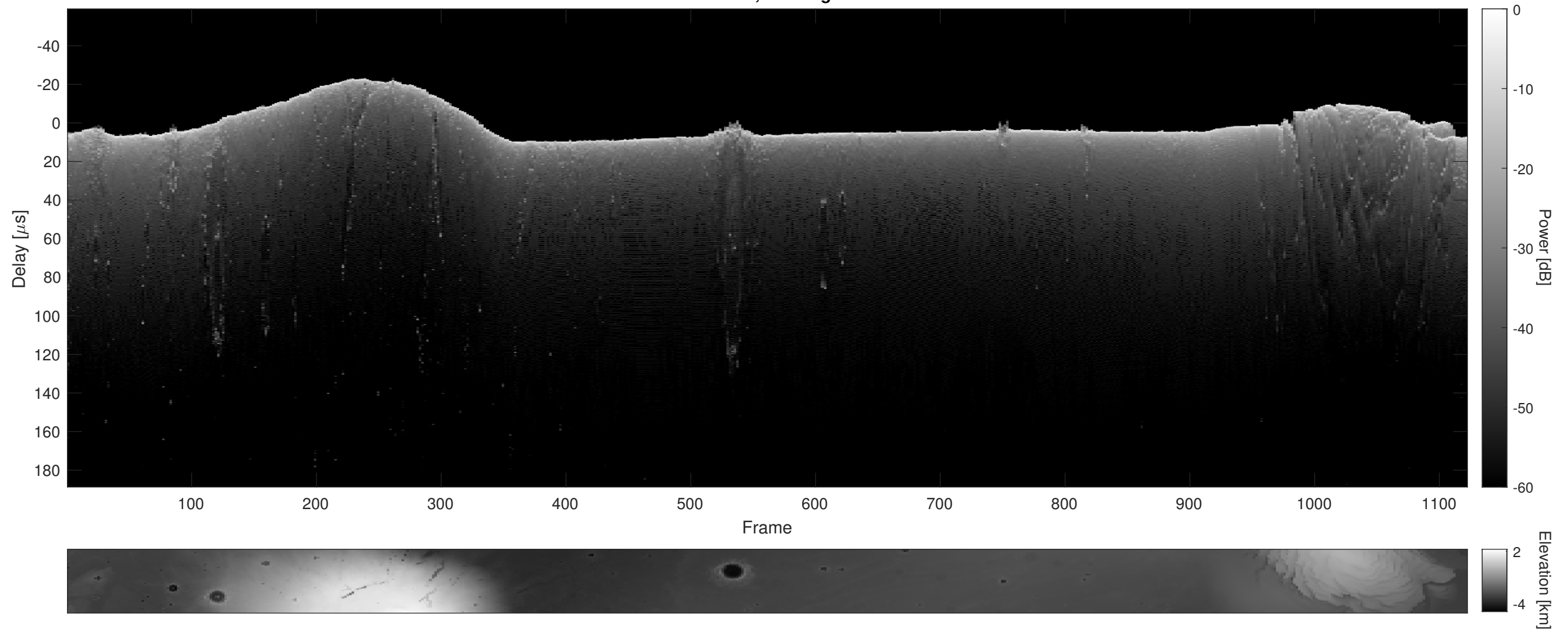
Orbit 3810, Cluttergram
