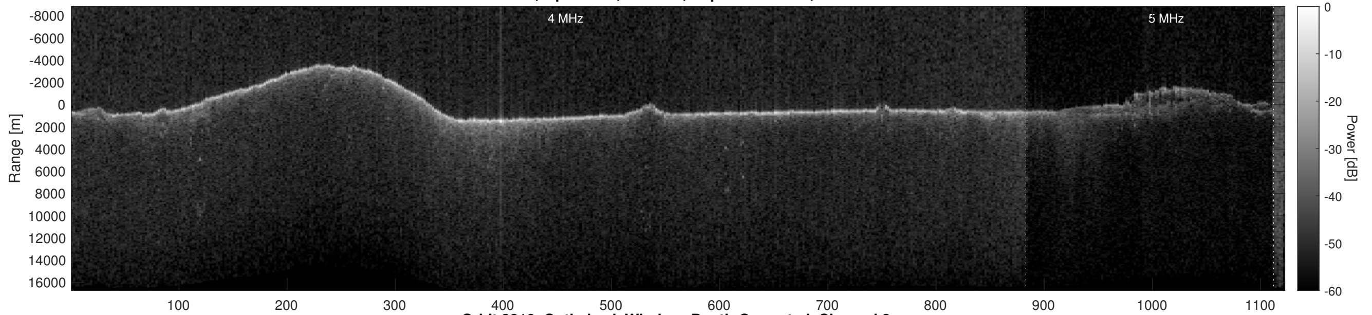
Orbit 3810, Optimized, Window, Depth-Corrected, Channel 2
