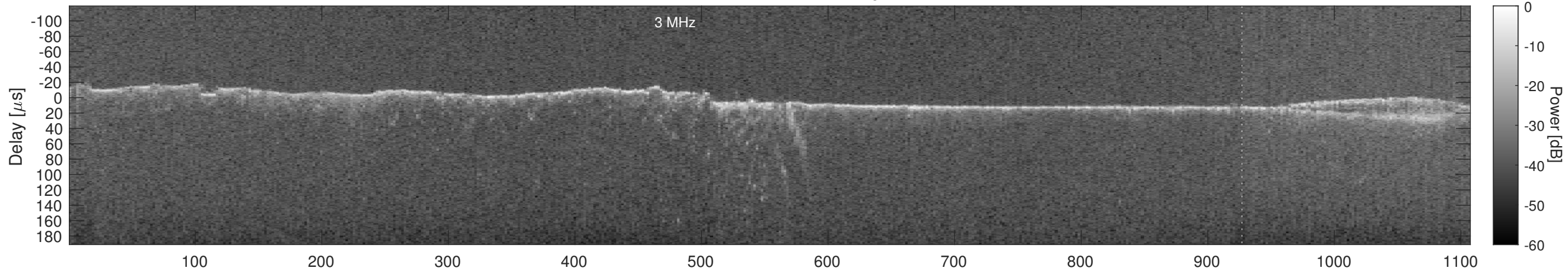
Orbit 3811, Cluttergram
