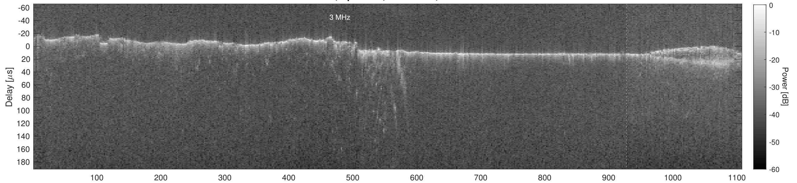
Orbit 3811, Cluttergram
