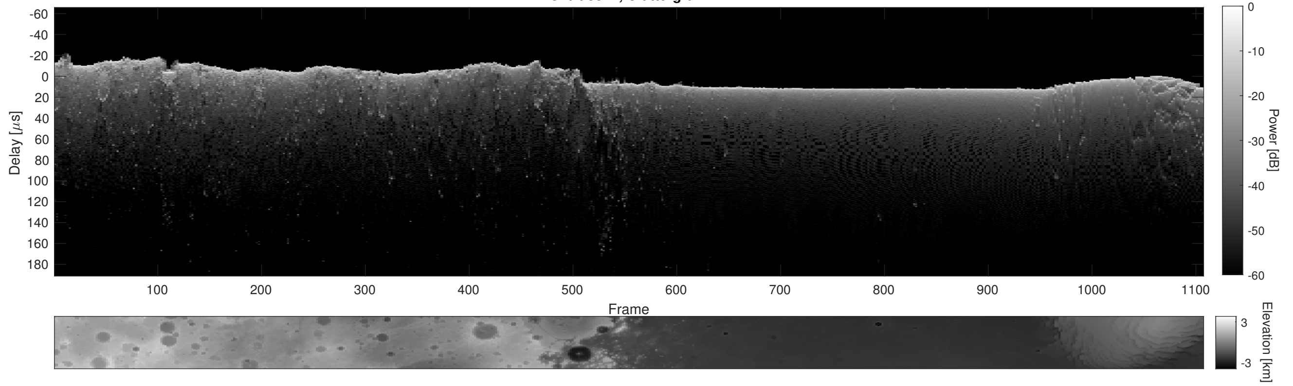
Orbit 3811, Cluttergram
