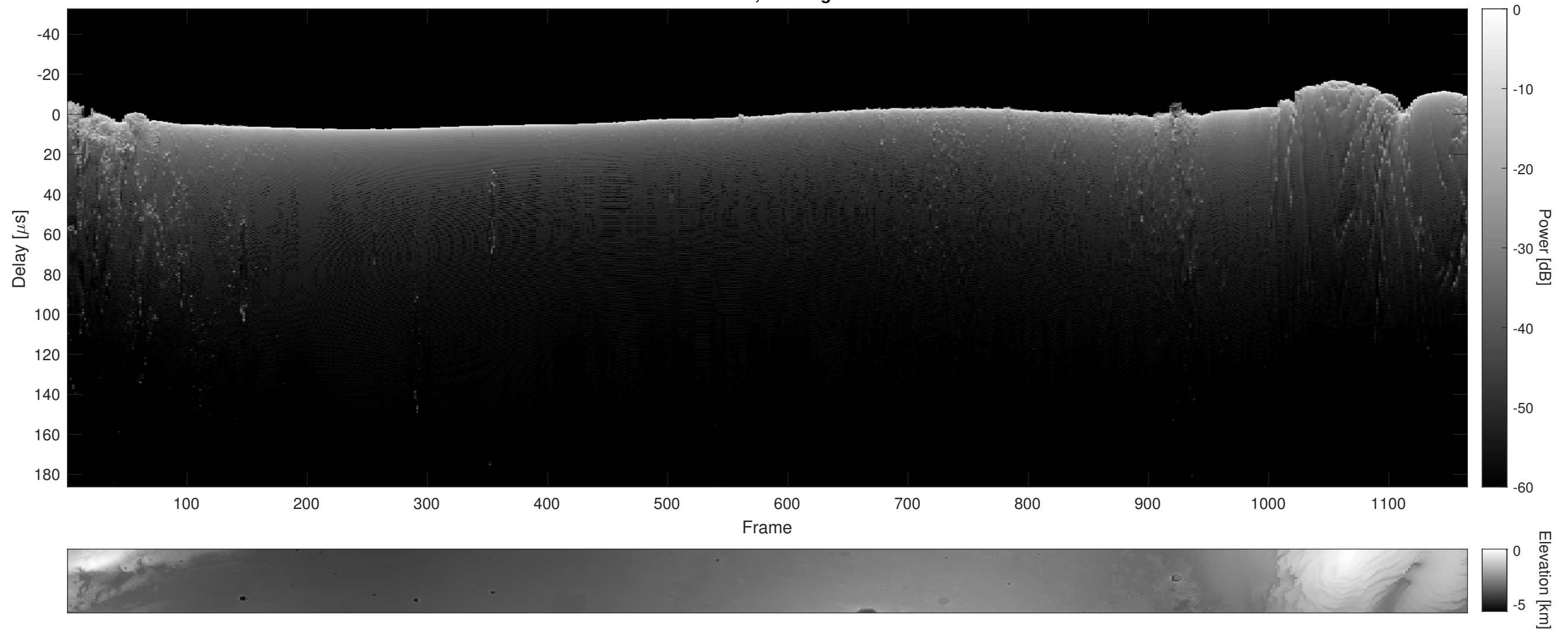
Orbit 3813, Cluttergram
