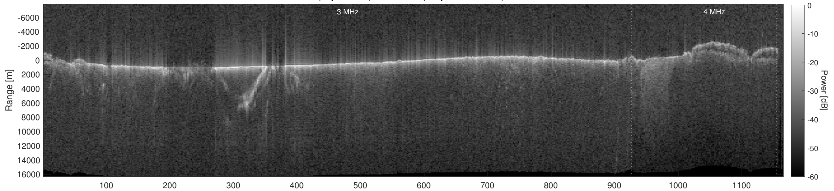
Orbit 3813, Depth-Corrected Cluttergram
