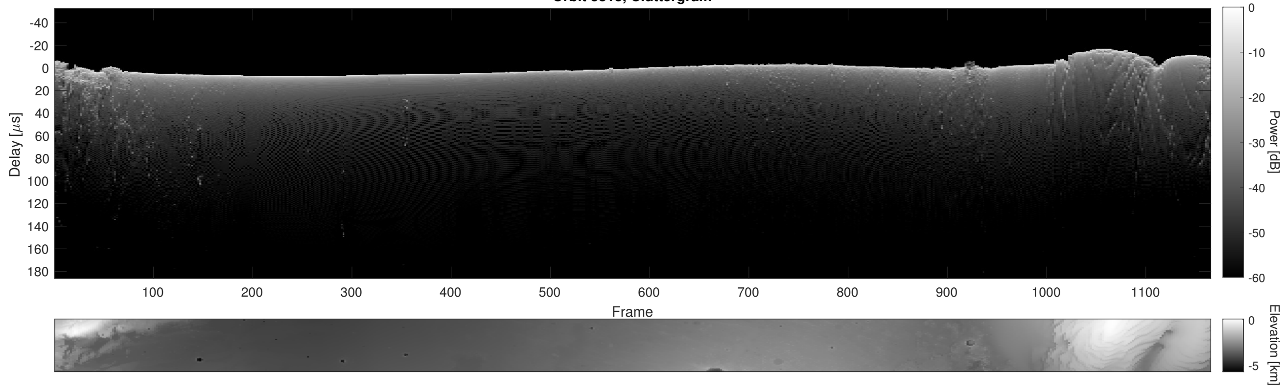
Orbit 3813, Cluttergram
