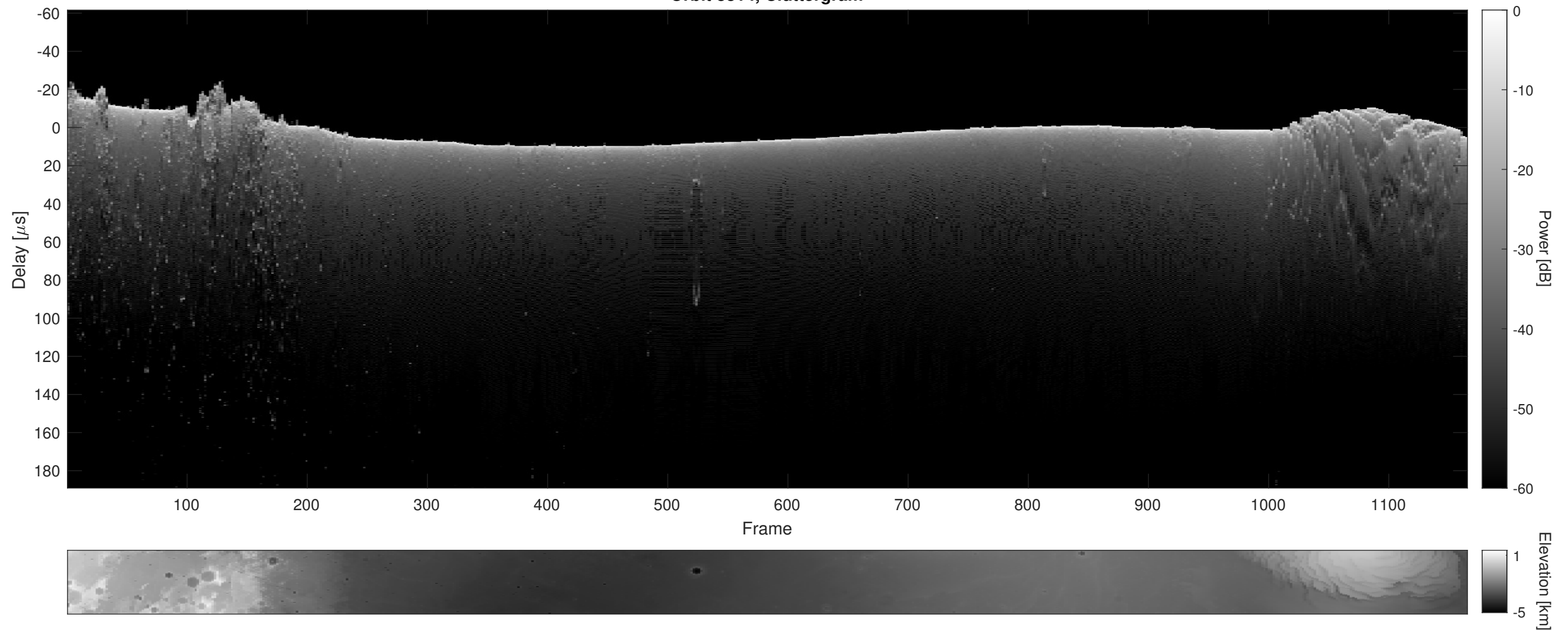
Orbit 3814, Cluttergram
