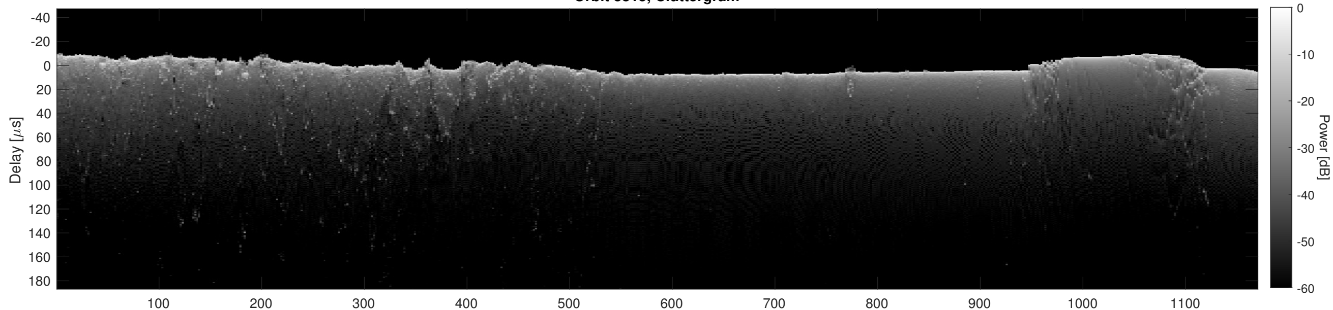
Orbit 3815, Cluttergram
