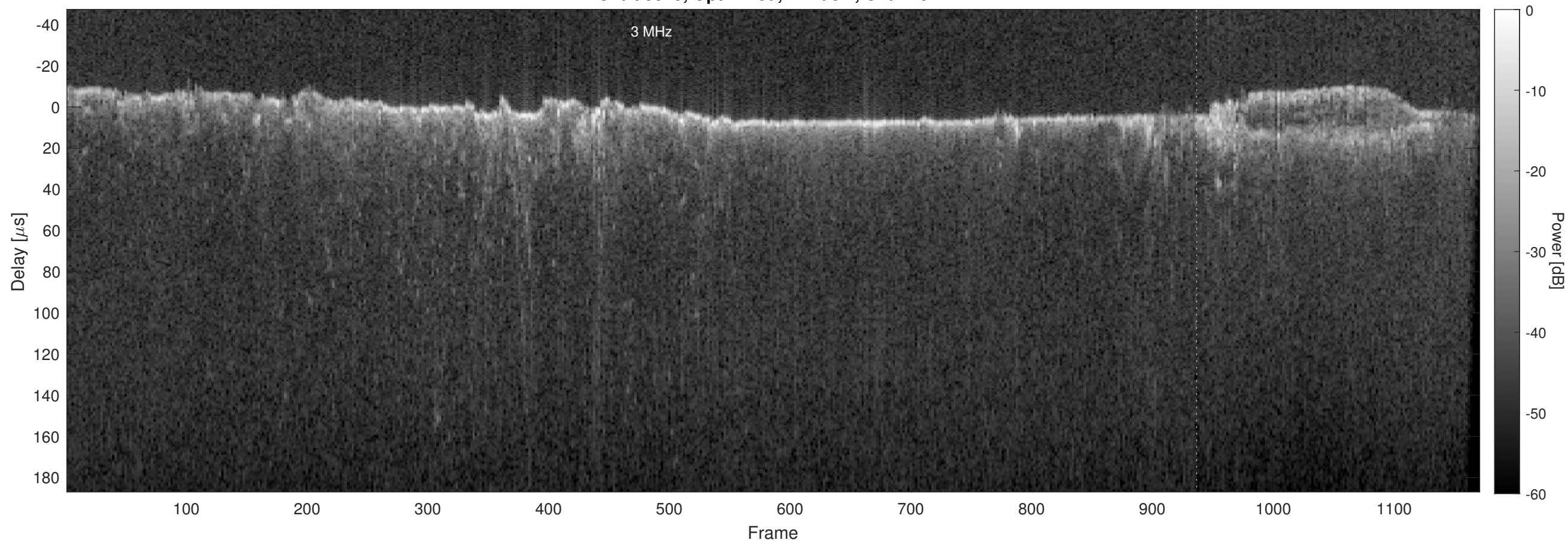
Orbit 3815, Optimized, Window, Channel 2
