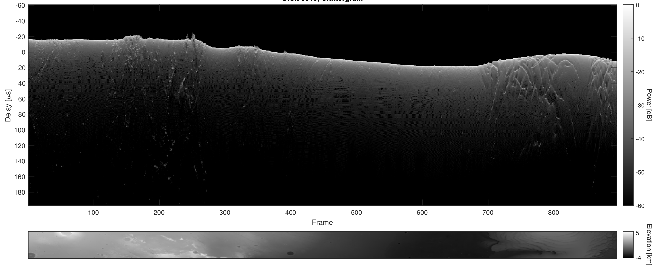
Orbit 3816, Cluttergram
