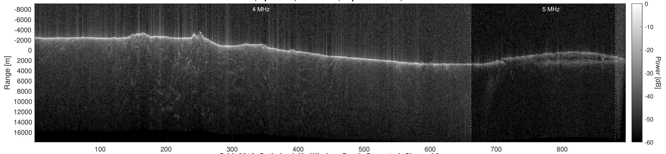
Orbit 3816, Optimized, No Window, Depth-Corrected, Channel 2
