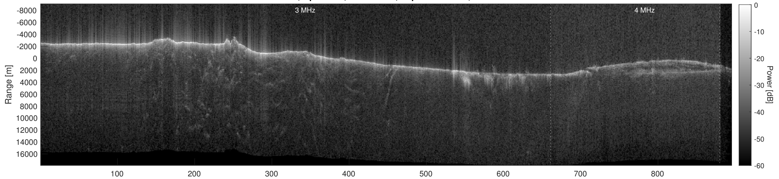
Orbit 3816, Depth-Corrected Cluttergram
