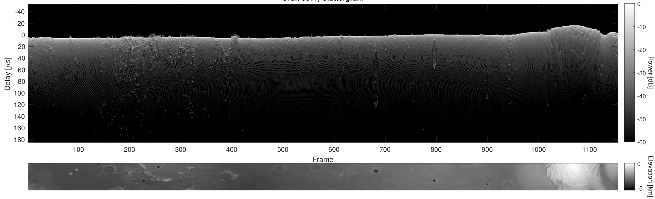
Orbit 3817, Cluttergram
