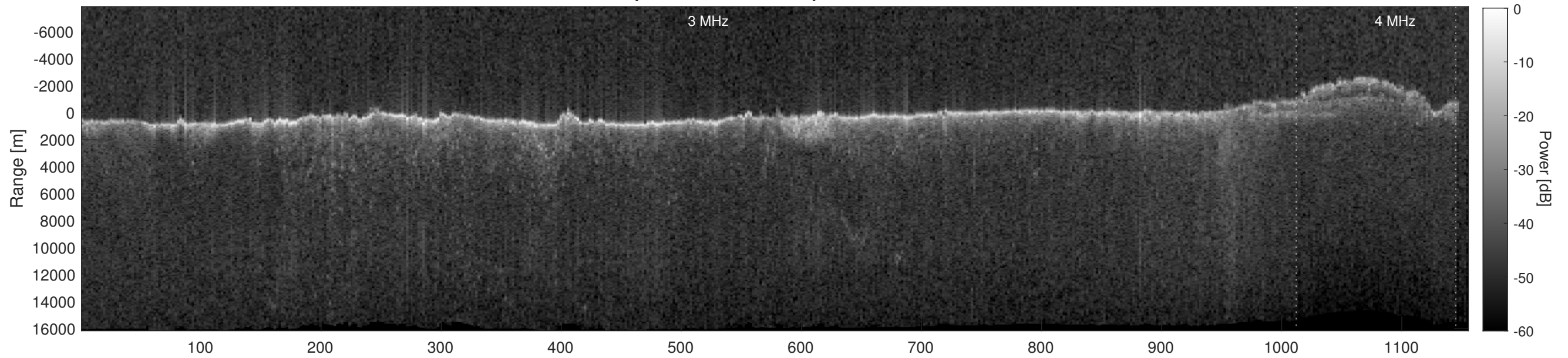
Orbit 3817, Depth-Corrected Cluttergram
