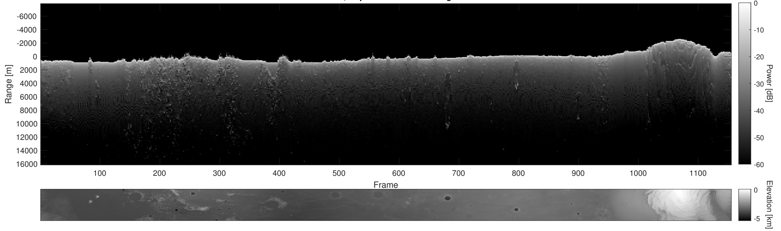
Orbit 3817, Depth-Corrected Cluttergram
