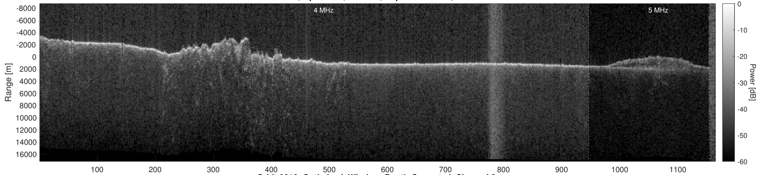
Orbit 3818, Optimized, Window, Depth-Corrected, Channel 2
