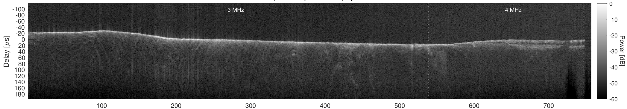
Orbit 3820, Cluttergram
