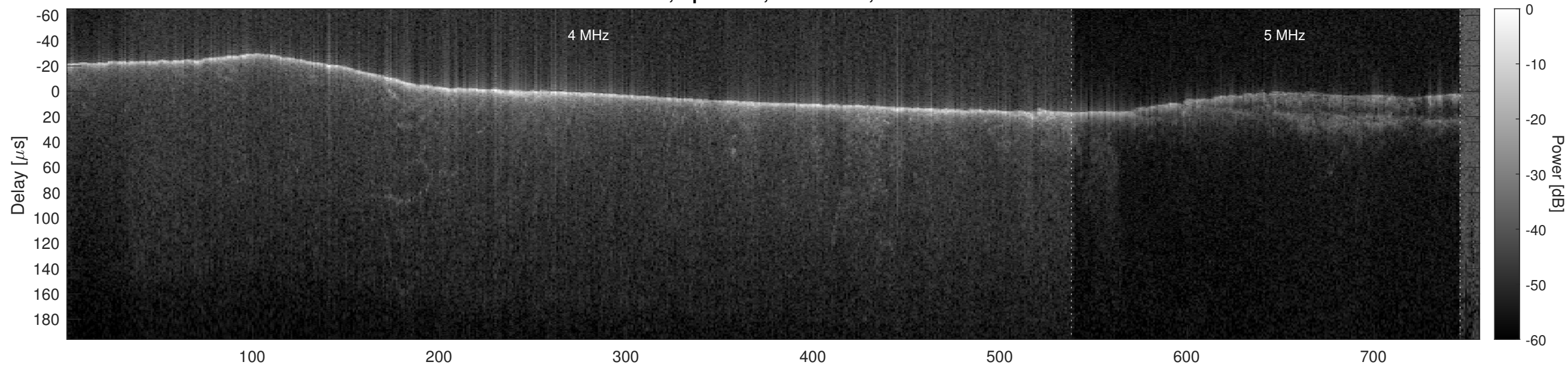
Orbit 3820, Optimized, No Window, Channel 2
