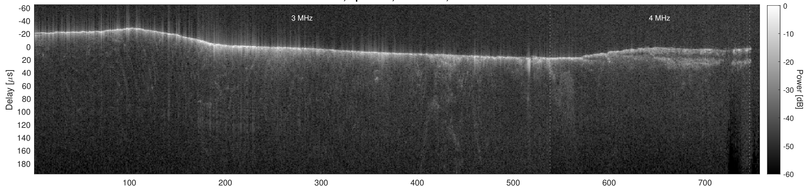
Orbit 3820, Cluttergram
