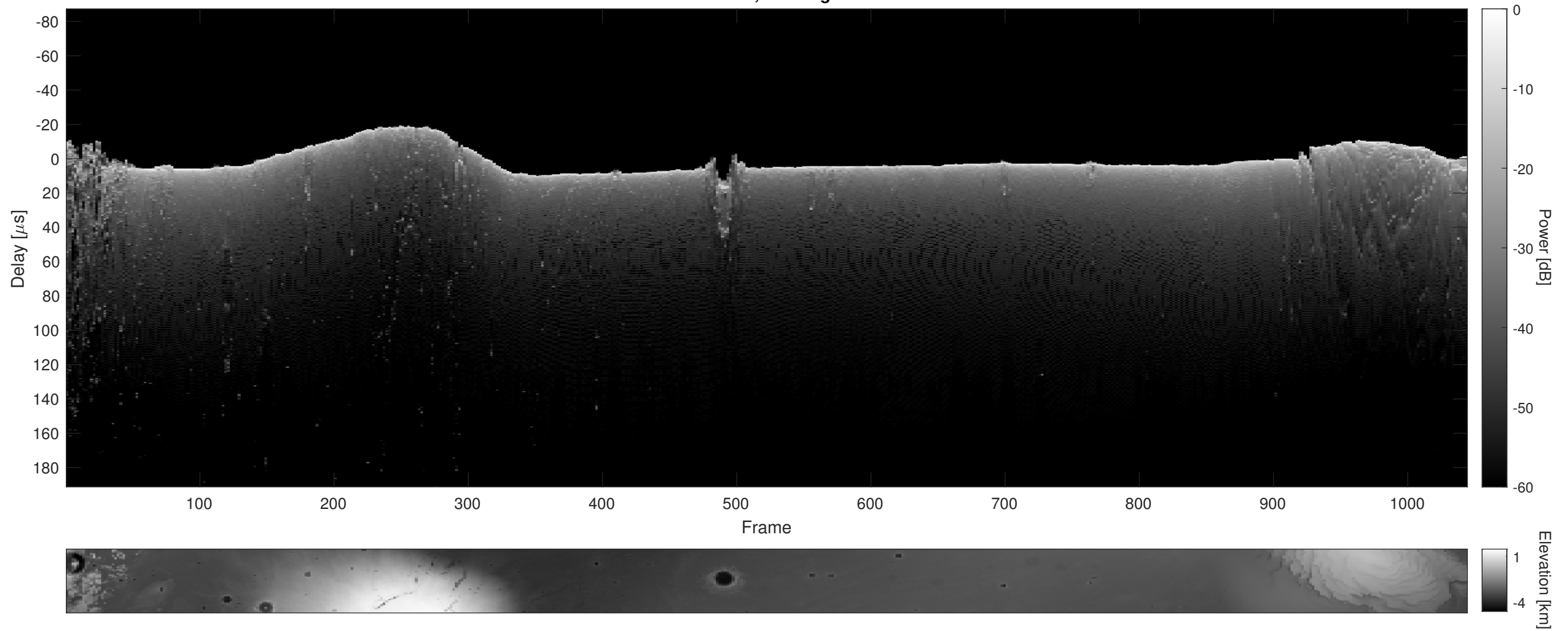
Orbit 3821, Cluttergram
