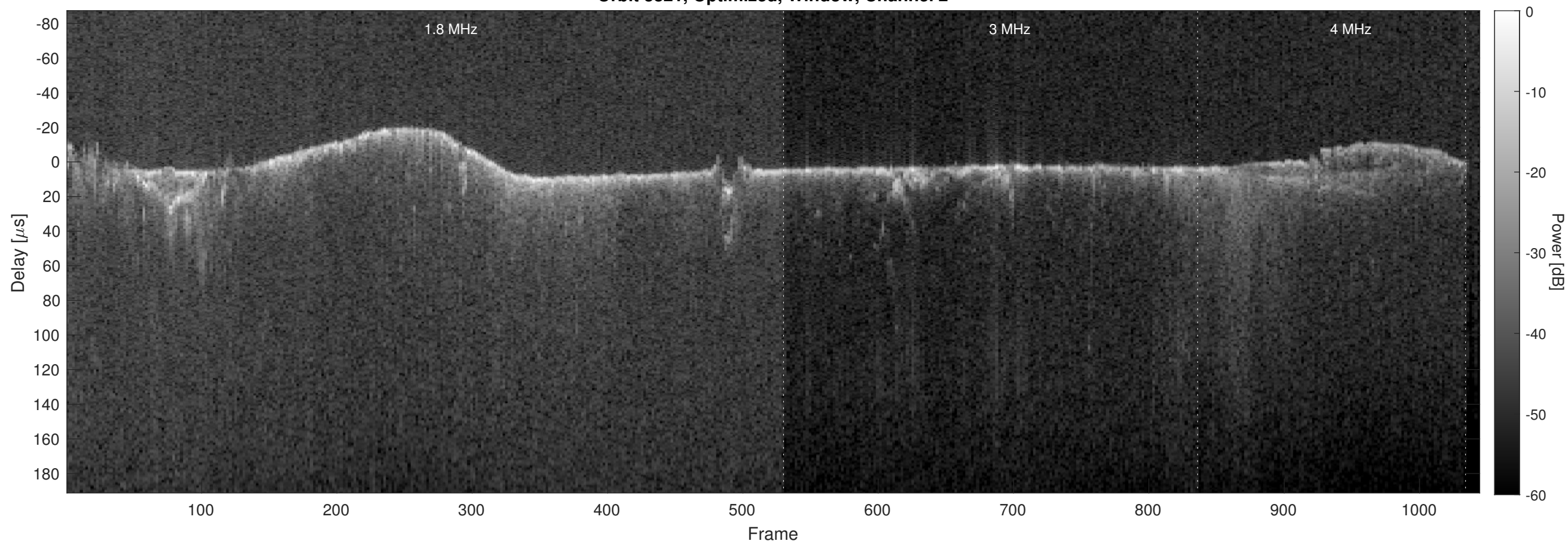
Orbit 3821, Optimized, Window, Channel 2
