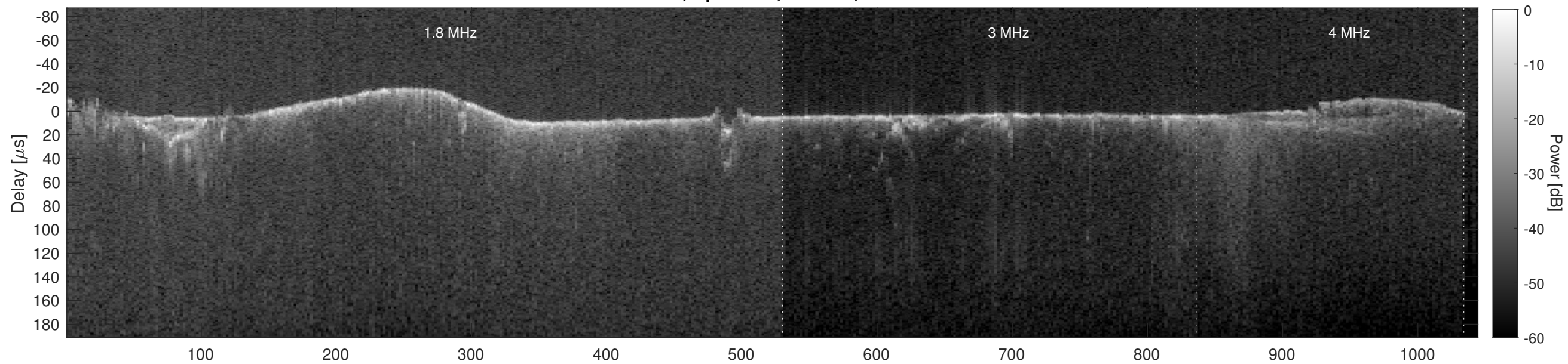
Orbit 3821, Cluttergram
