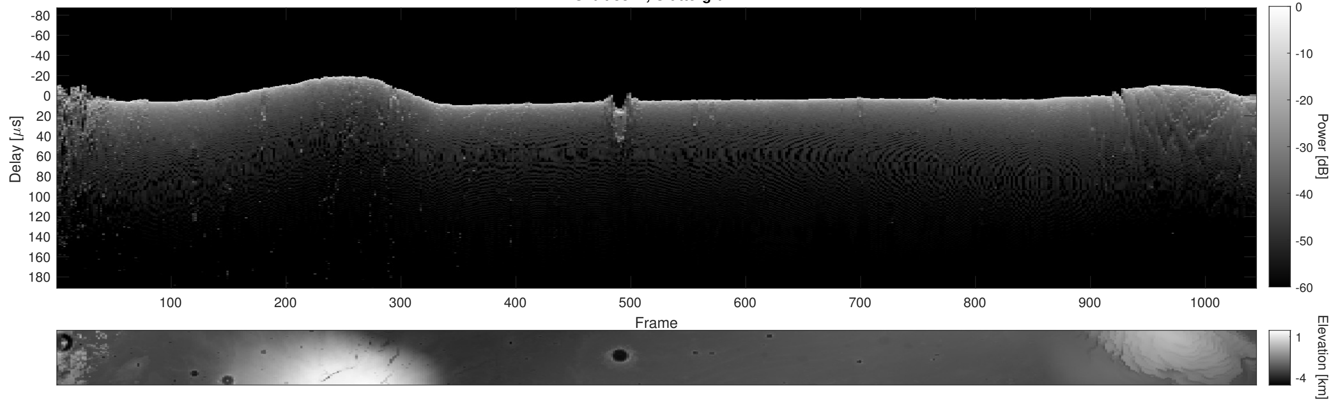
Orbit 3821, Cluttergram
