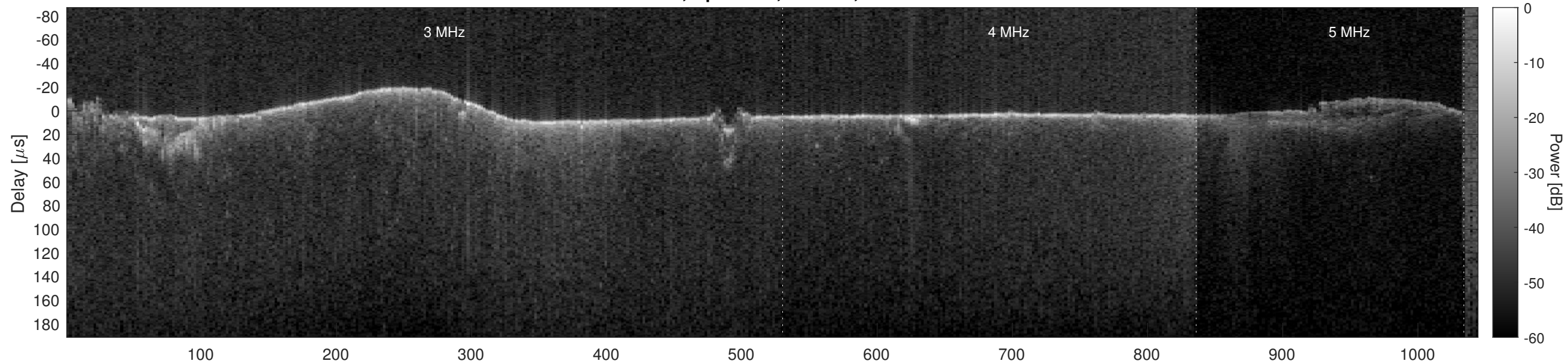
Orbit 3821, Optimized, Window, Channel 2
