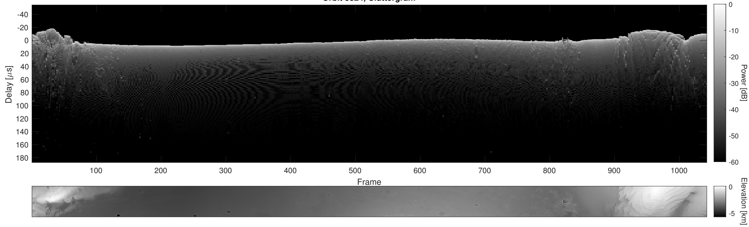
Orbit 3824, Cluttergram
