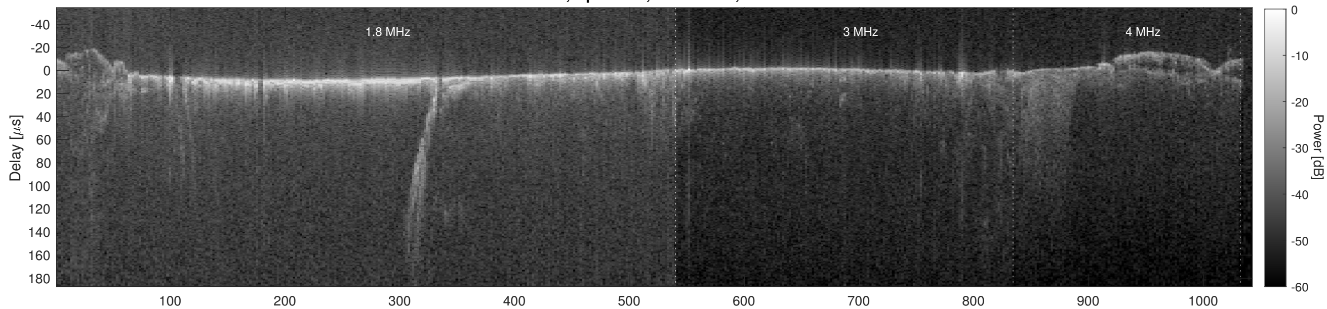
Orbit 3824, Cluttergram
