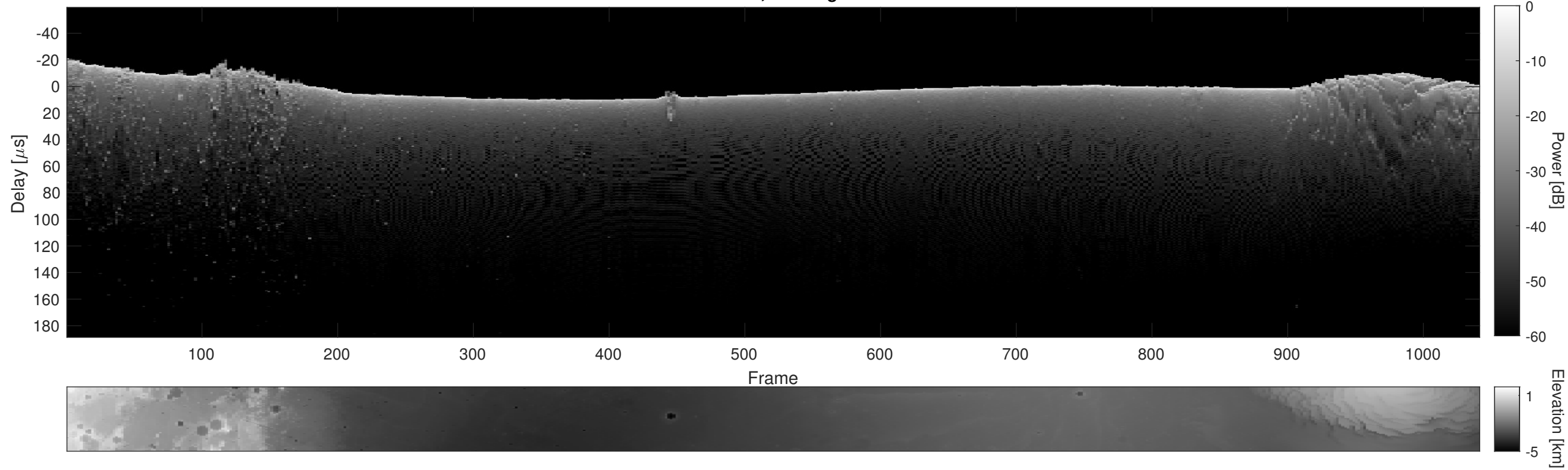
Orbit 3825, Cluttergram
