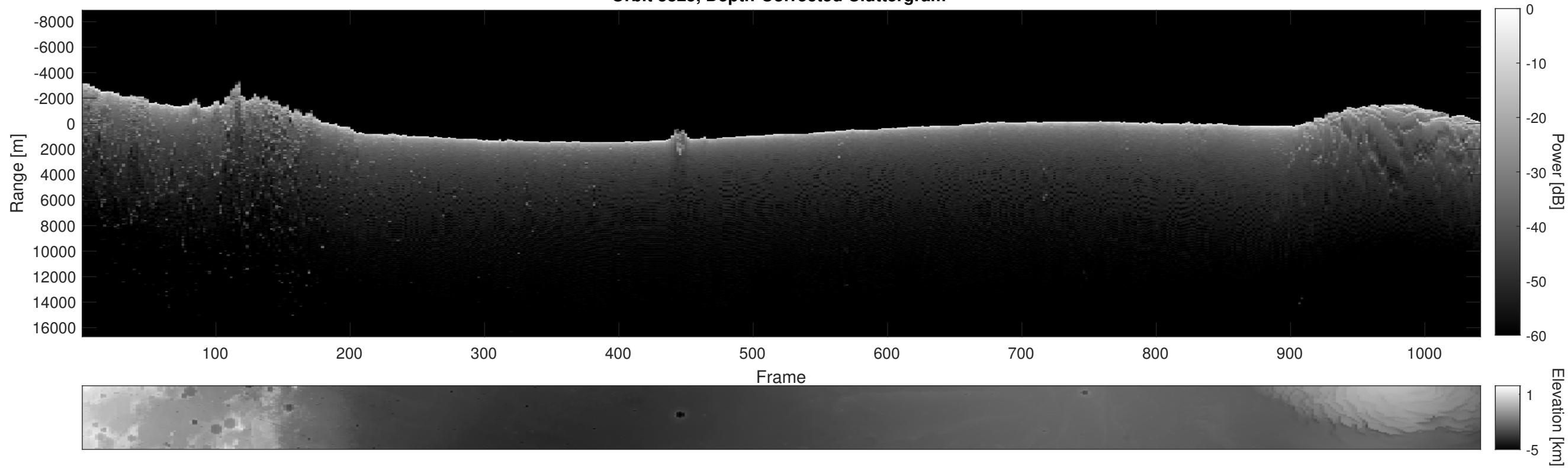
Orbit 3825, Depth-Corrected Cluttergram
