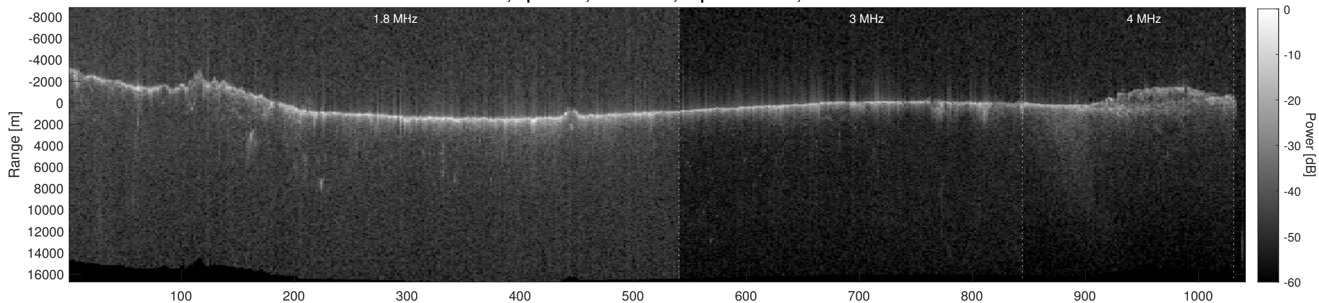
Orbit 3825, Depth-Corrected Cluttergram
