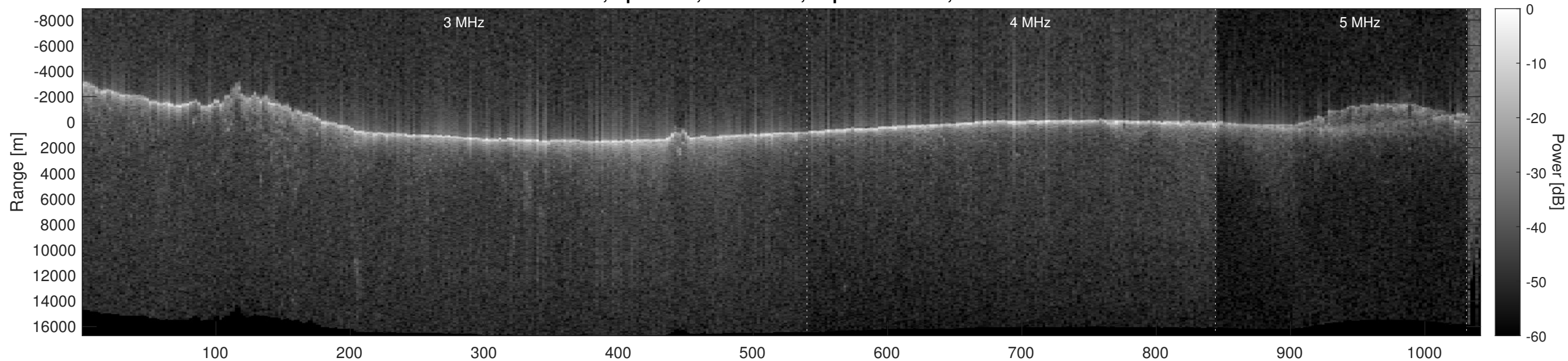
Orbit 3825, Optimized, No Window, Depth-Corrected, Channel 2
